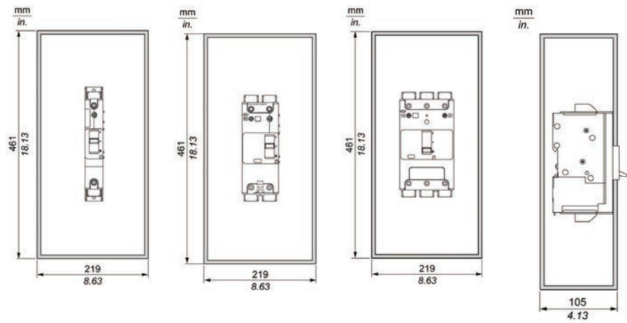
1P Front View
